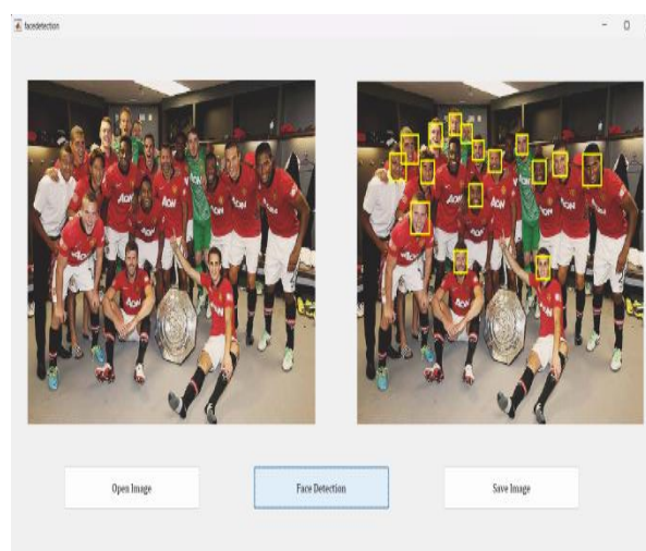
Figure 8. Face detection
