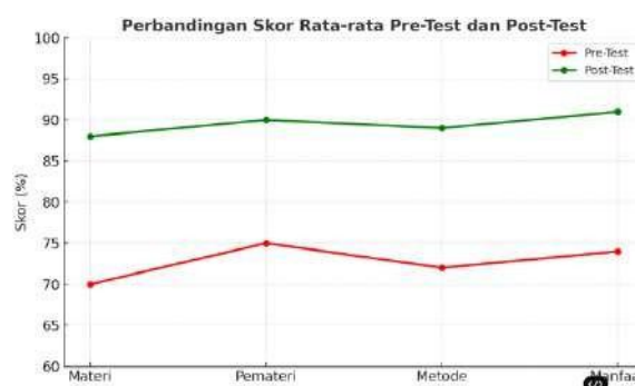
Graph 1. Participants' Average Pre-test and Post-test Scores
